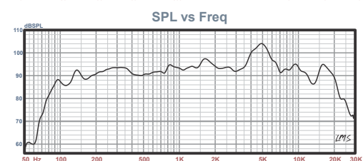
Response curve obtained in a 8L x 110Hz box (1W x 1m).
