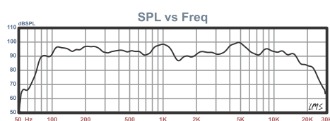
Response curve obtained in a 10L x 105Hz box (1W x 1m).
